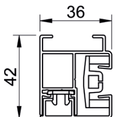
glissière ZIP "clips" 42mm P x 36mm L
